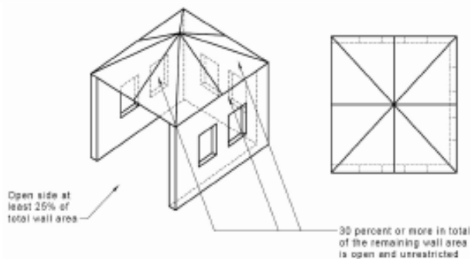
FIGURE E5—OUTDOOR AREA—EXAMPLE 5
