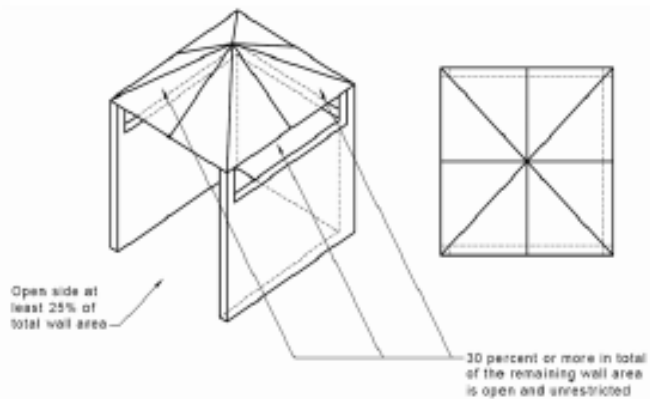
FIGURE E4—OUTDOOR AREA—EXAMPLE 4
