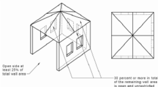
FIGURE E3—OUTDOOR AREA—EXAMPLE 3
