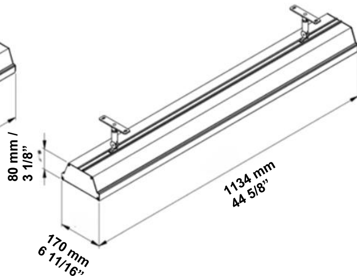
X- THX6000DC
